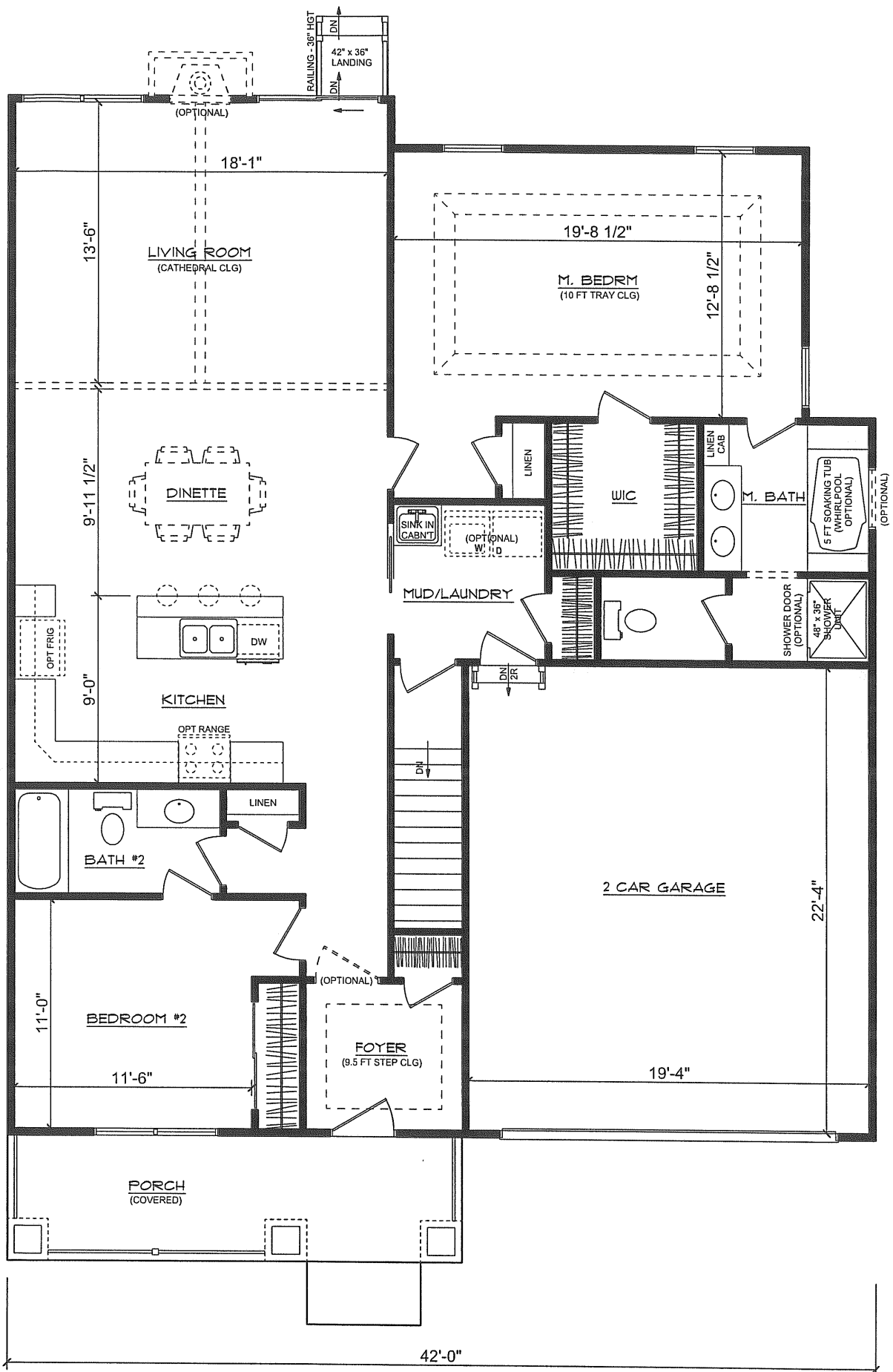
FIRST FLOOR PLAN Burke Darwin Model
