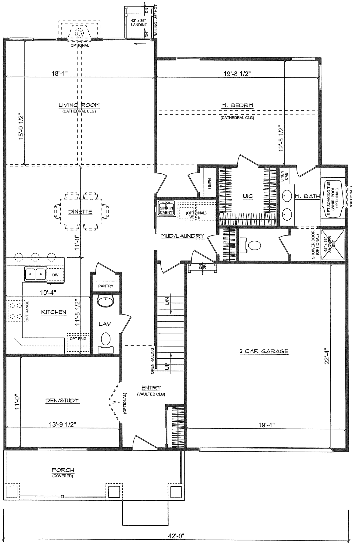
FIRST FLOOR PLAN Burke Cambridge Model
