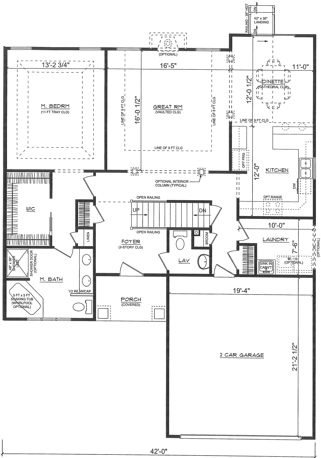
FIRST FLOOR PLAN Burke Andover Model
