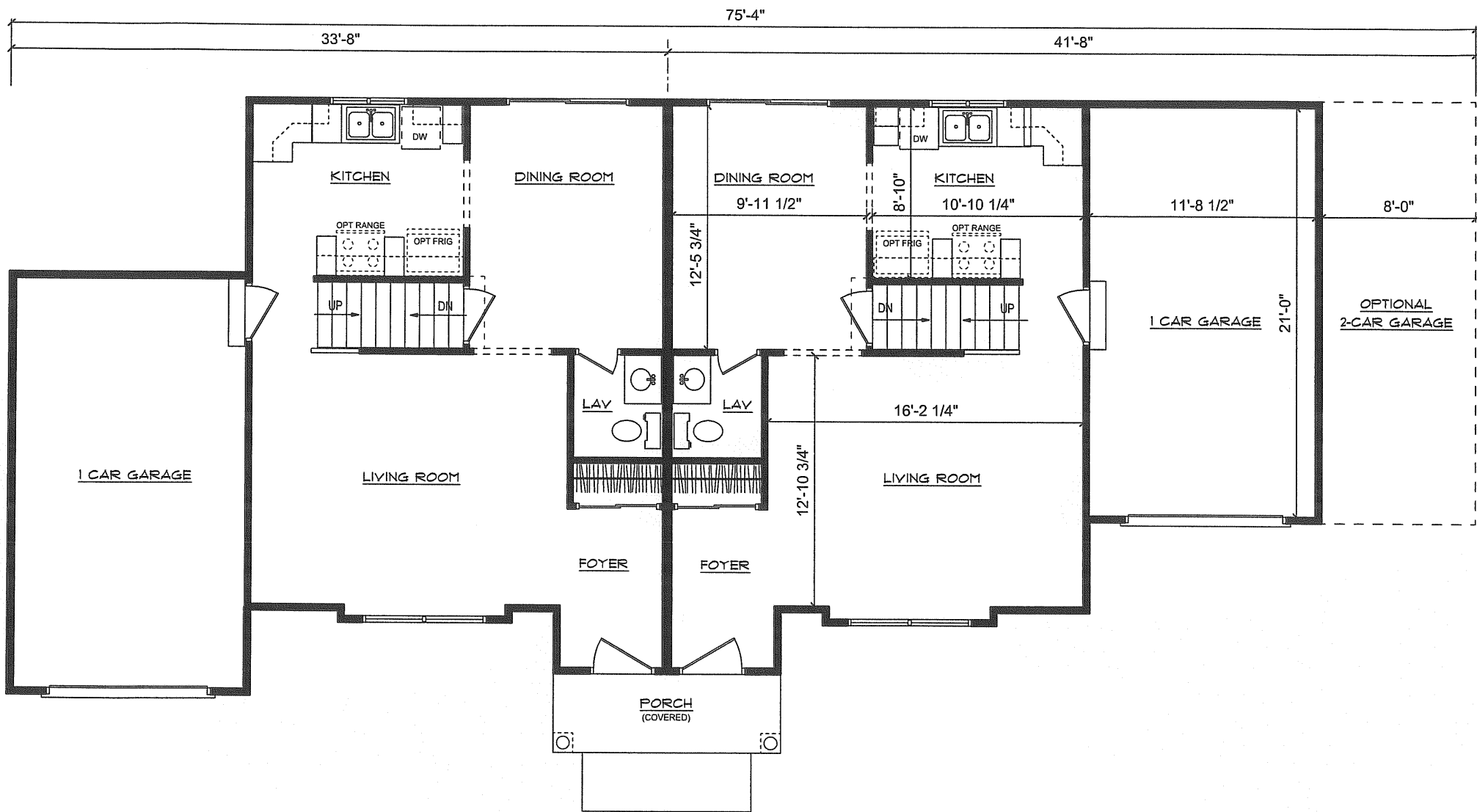
FIRST FLOOR PLAN BURKE QUINCY MODEL OAKWOOD TOWNHOMES
