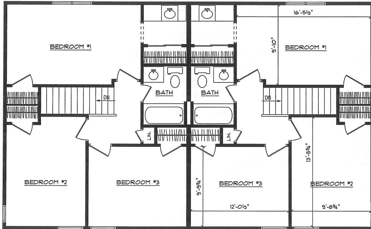
SECOND FLOOR PLAN BURKE QUINCY MODEL OAKWOOD TOWNHOMES
