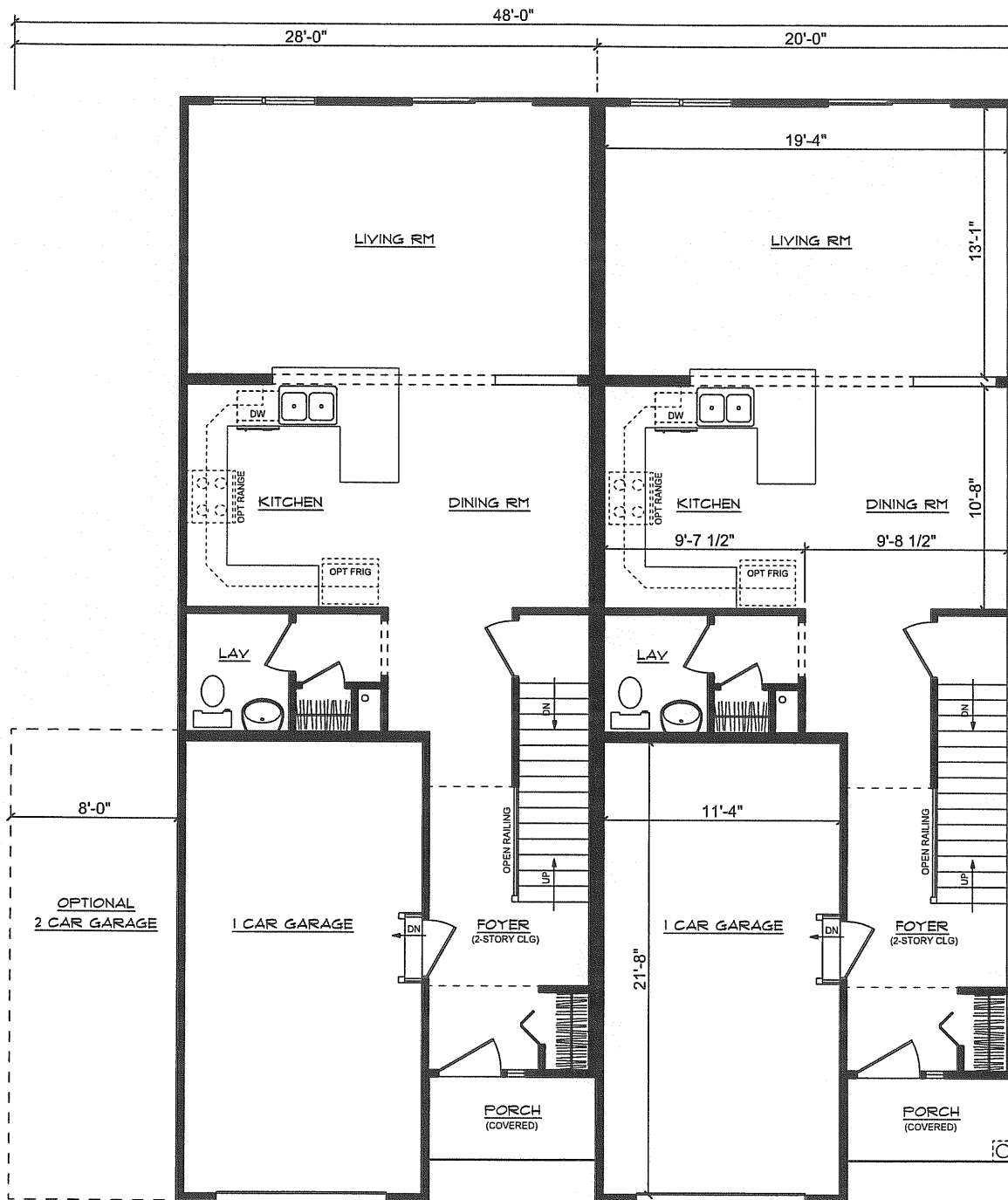
FIRST FLOOR PLAN BURKE HUNTINGTON MODEL OAKWOOD TOWNHOMES
