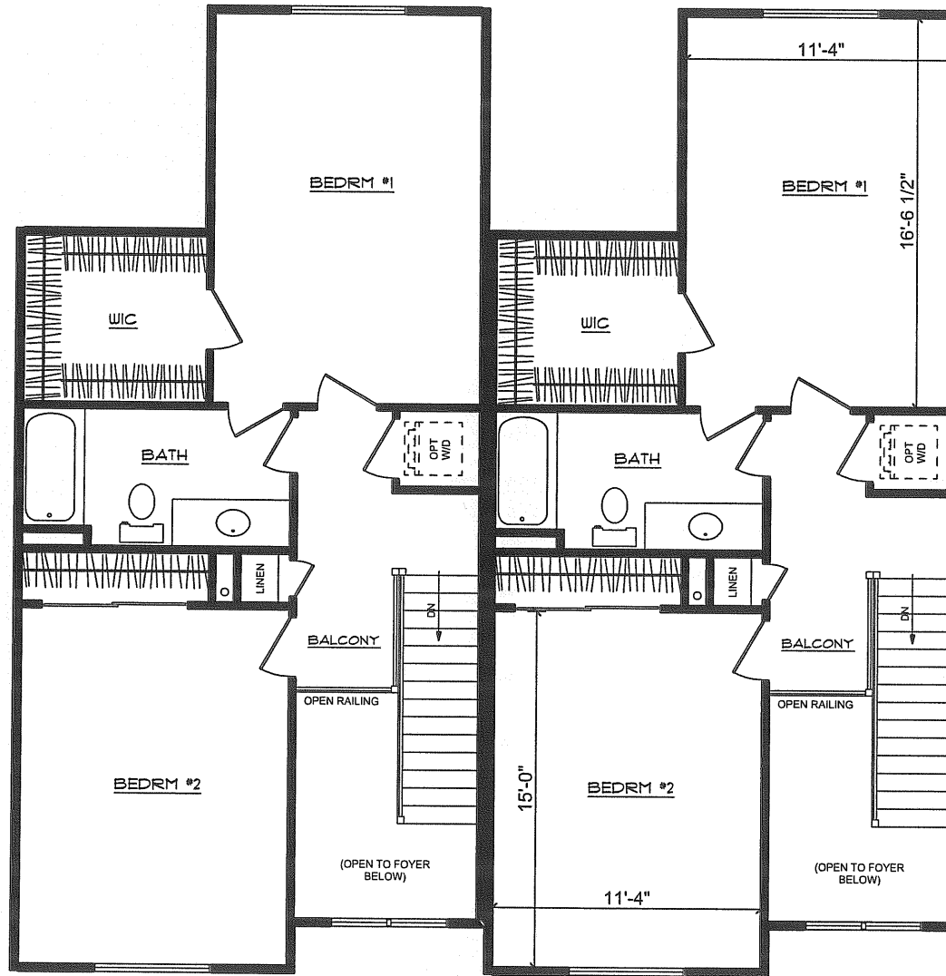
SECOND FLOOR PLAN BURKE HUNTINGTON MODEL OAKWOOD TOWNHOMES
