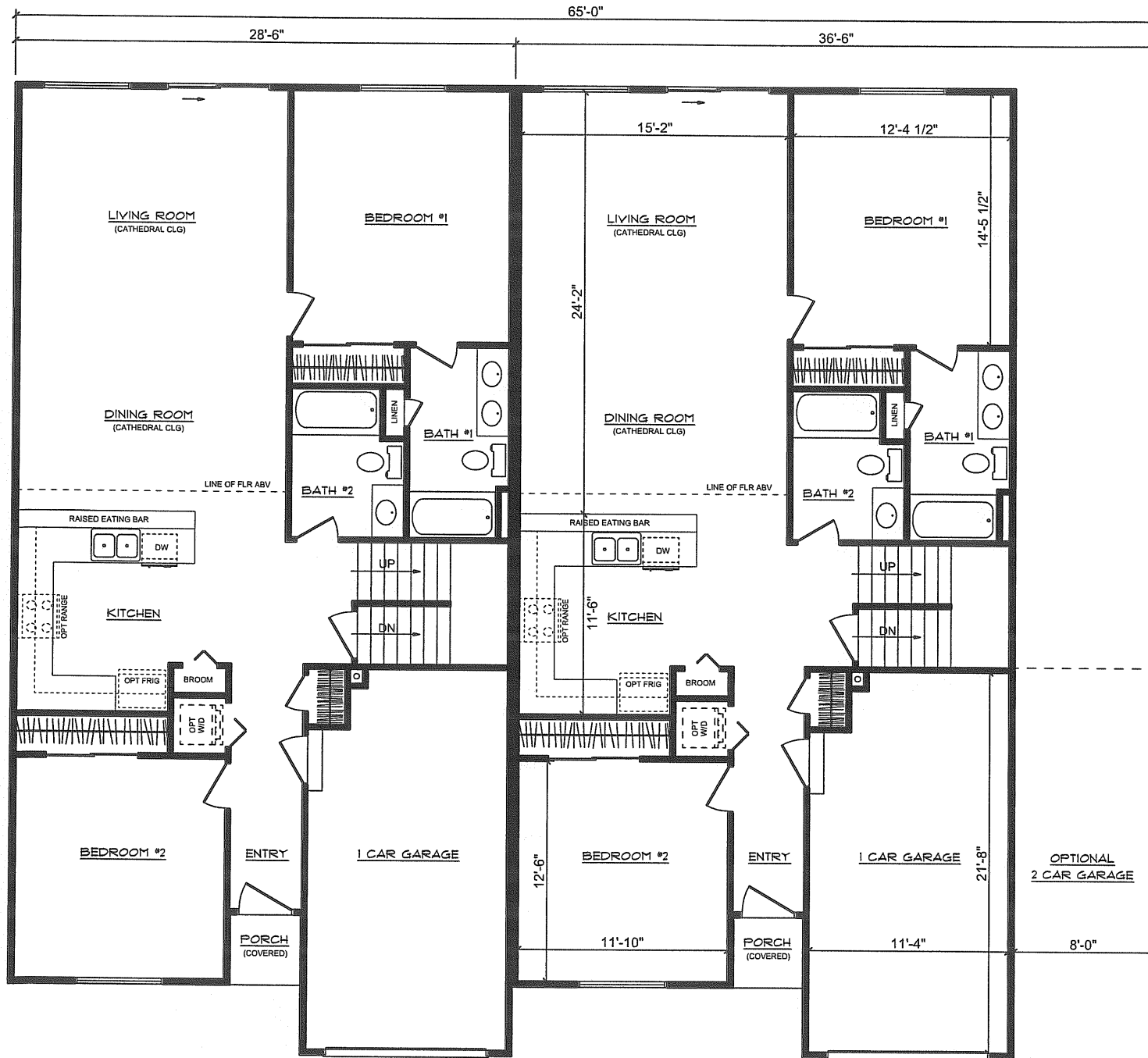
FIRST FLOOR PLAN BURKE DURHAM MODEL OAKWOOD TOWNHOMES
