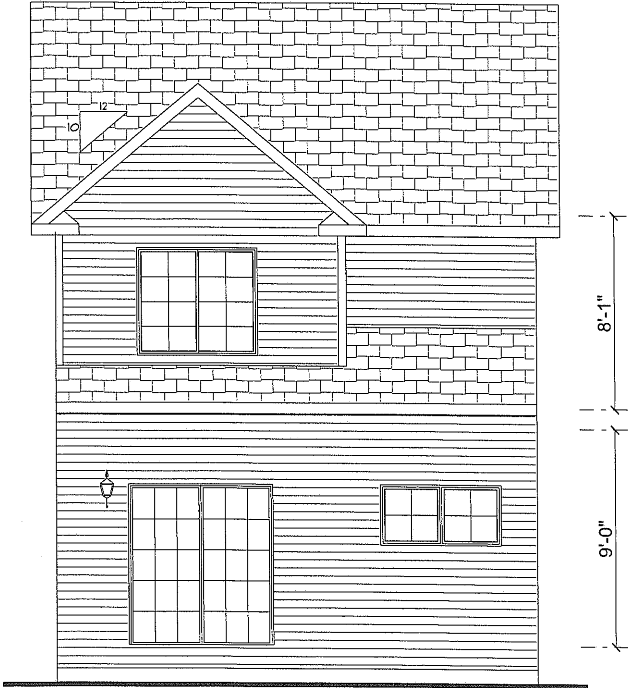
REAR ELEVATION BROOKSIDE VILLAGE TOWNHOMES TYPICAL HUNTINGTON (B) MODEL
