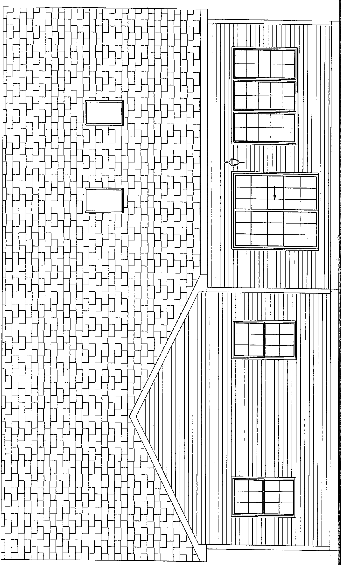
REAR ELEVATION BROOKSIDE VILLAGE TOWNHOUSE 1-STORY W/LOFT, 'E' UNIT
