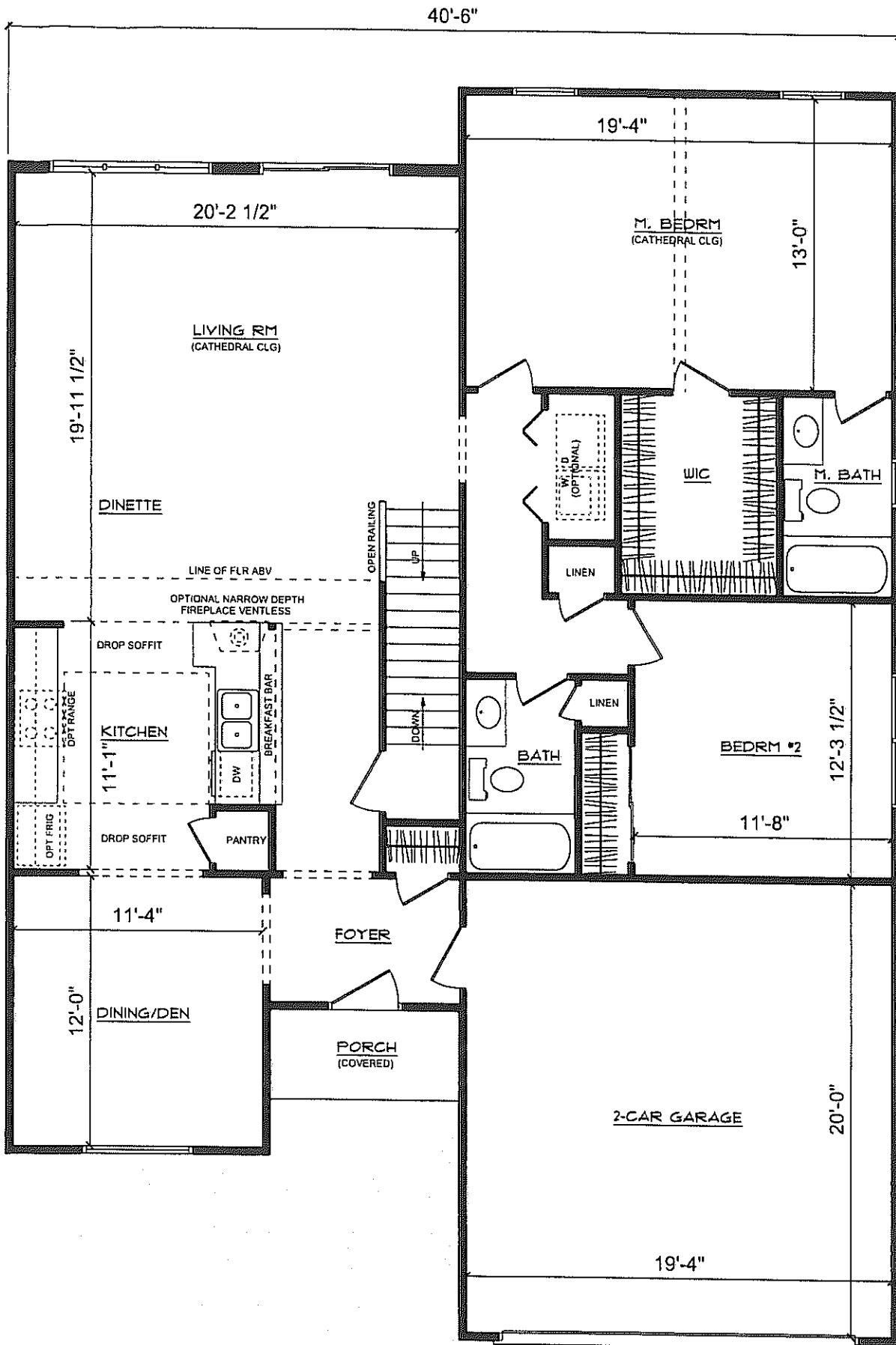
FLOOR PLAN = 1,560.0 SF BROOKSIDE VILLAGE TOWNHOUSE - BLDG #4 1-STORY W/LOFT, E UNIT PLAN
