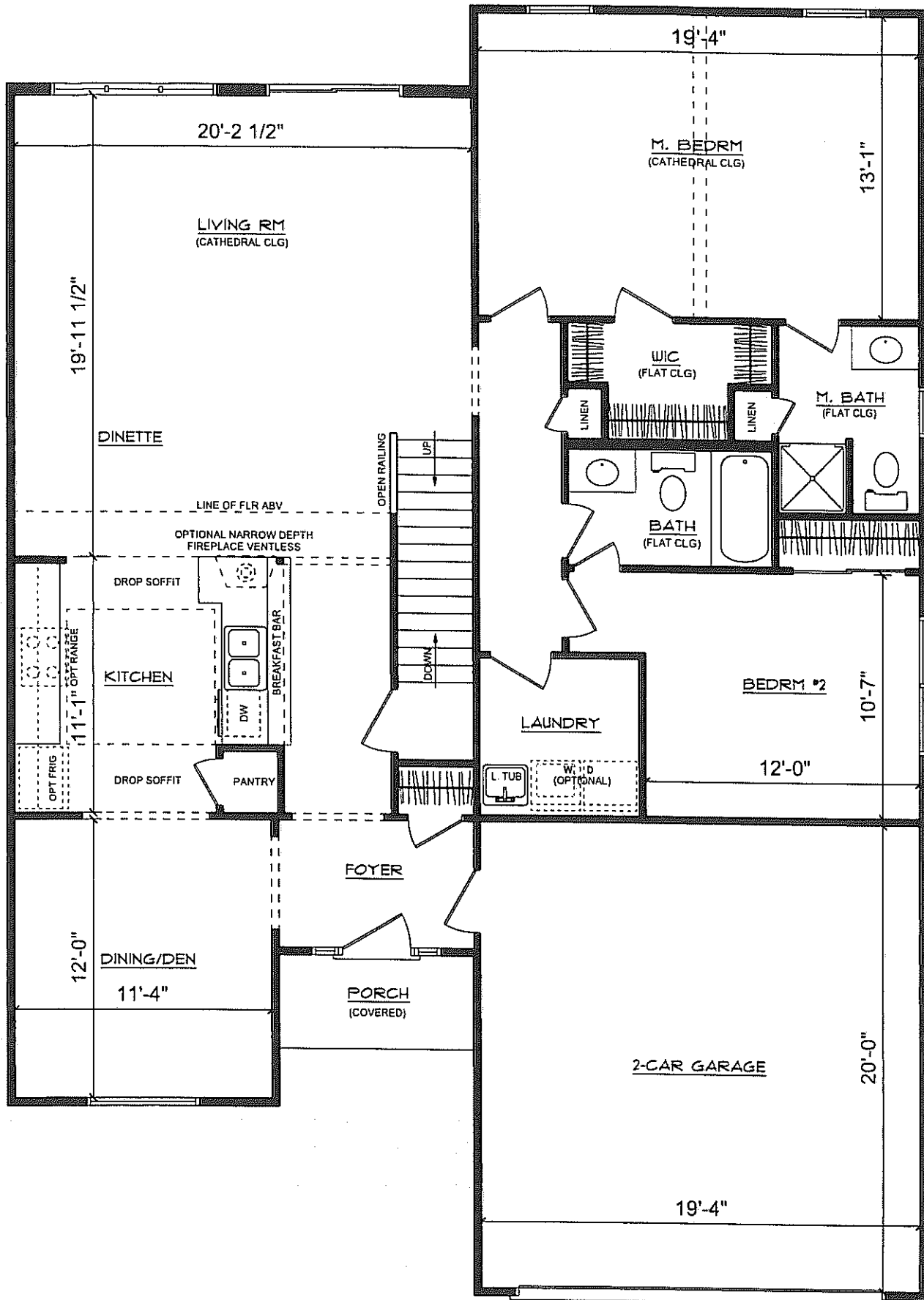
ALT FLOOR PLAN = 1,560.0 SF BROOKSIDE VILLAGE TOWNHOUSE - BLDG #4 1-STORY W/LOFT, E UNIT PLAN
