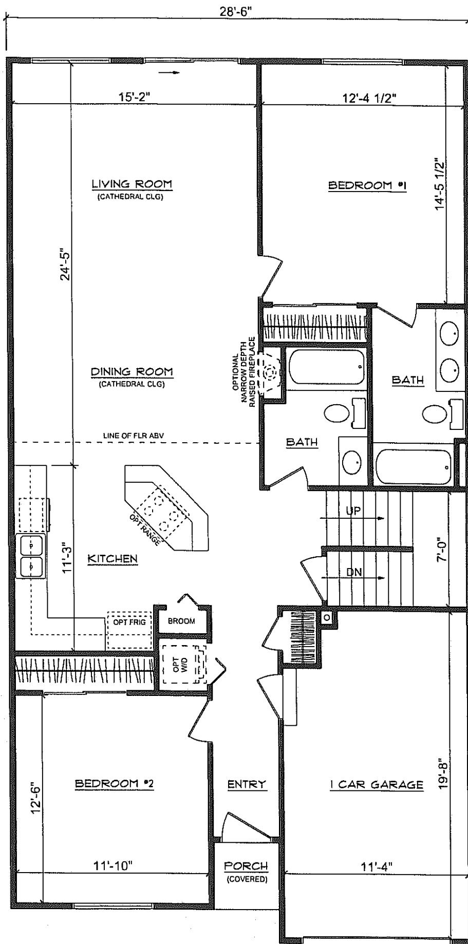
FLOOR PLAN = 1,249.0 SF BROOKSIDE VILLAGE TOWNHOUSE - BLDG #3 1-STORY W/LOFT, 'D' UNIT PLAN
