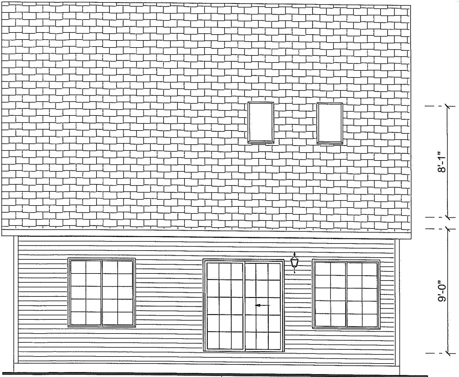
REAR ELEVATION BROOKSIDE VILLAGE TOWNHOUSE 1-STORY W/LOFT, 'D' UNIT
