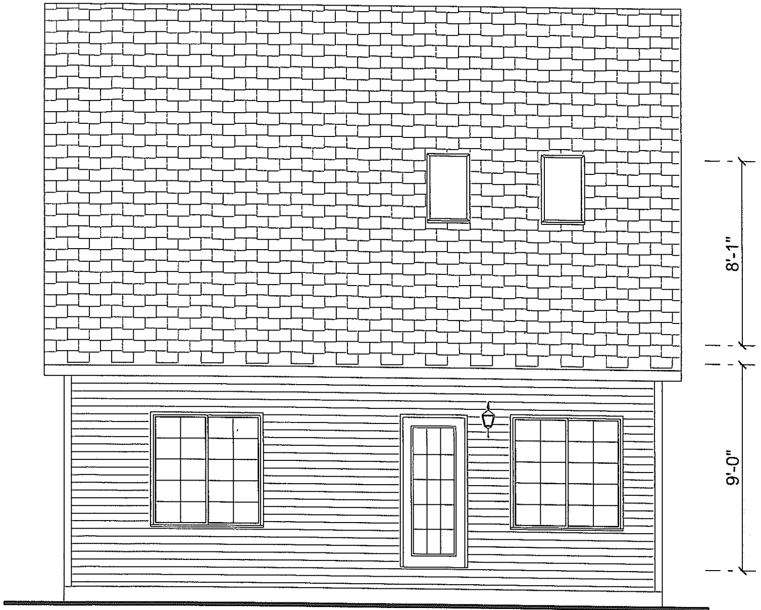
REAR ELEVATION BROOKSIDE VILLAGE TOWNHOUSE 1-STORY W/LOFT, 'C' UNIT
