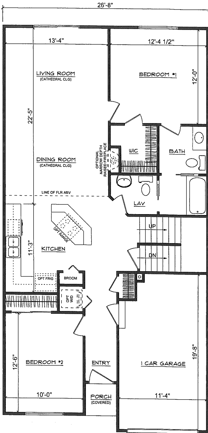
FLOOR PLAN = 1,100.0 SF BROOKSIDE VILLAGE TOWNHOUSE - BLDG #2 1-STORY W/LOFT, 'C' UNIT PLAN
