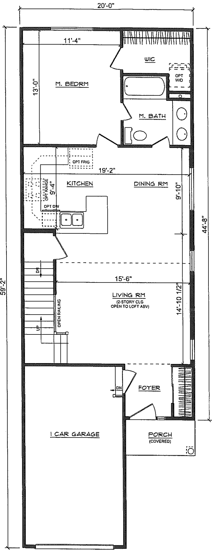
FIRST FLOOR PLAN AMBERWOOD (AE) MODEL BSVT / REV #: 5 / 27 JAN 09
