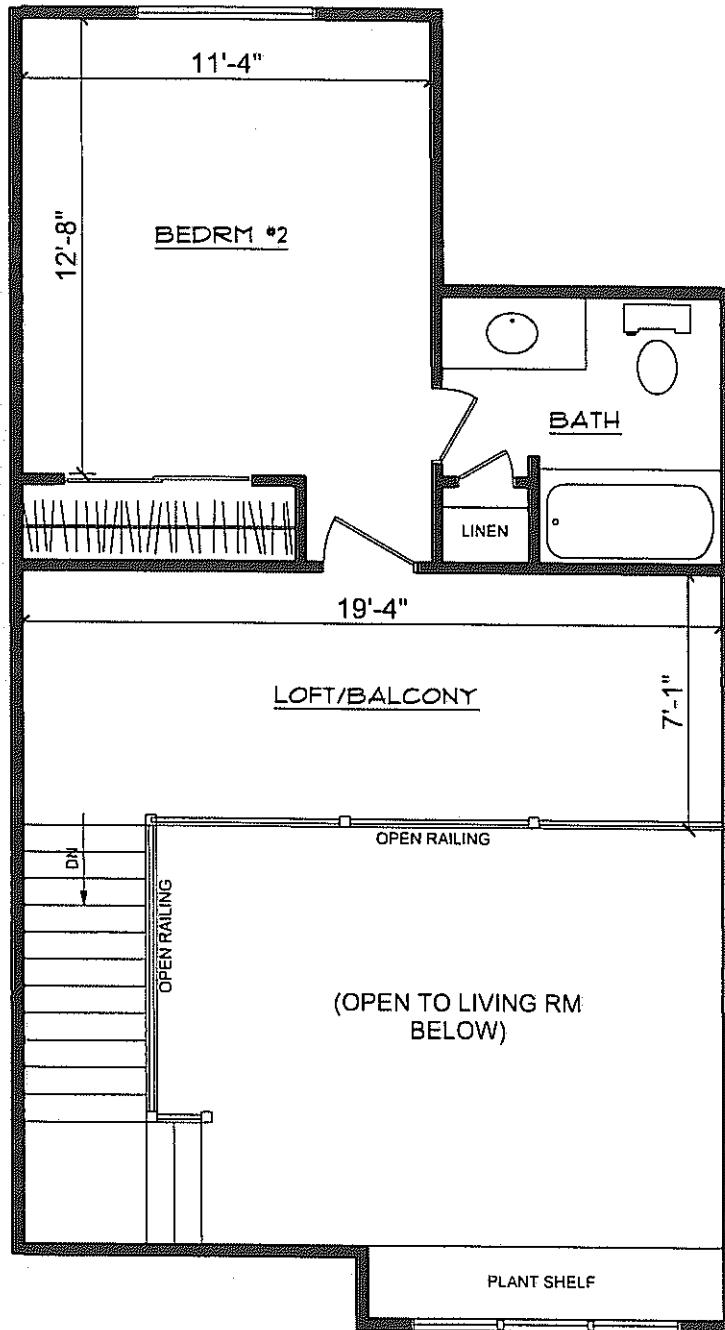
SECOND FLOOR PLAN AMBERWOOD (AE) MODEL BSVT / REV #: 5 / 27 JAN 09
