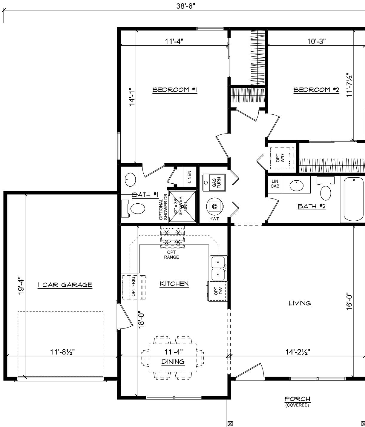
FLOOR PLAN BURKE ADDISON RANCH
