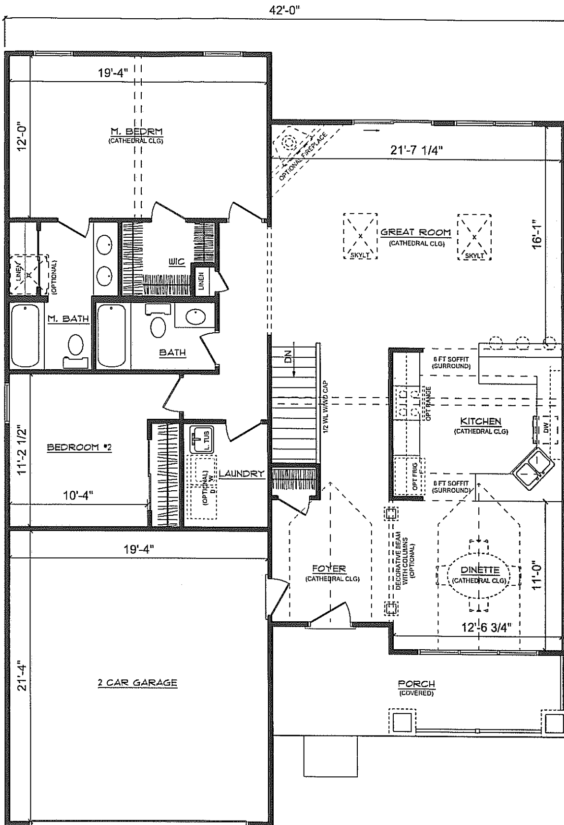
FIRST FLOOR PLAN BURKE EASTWOOD MODEL BROMPTON TOWNHOMES
