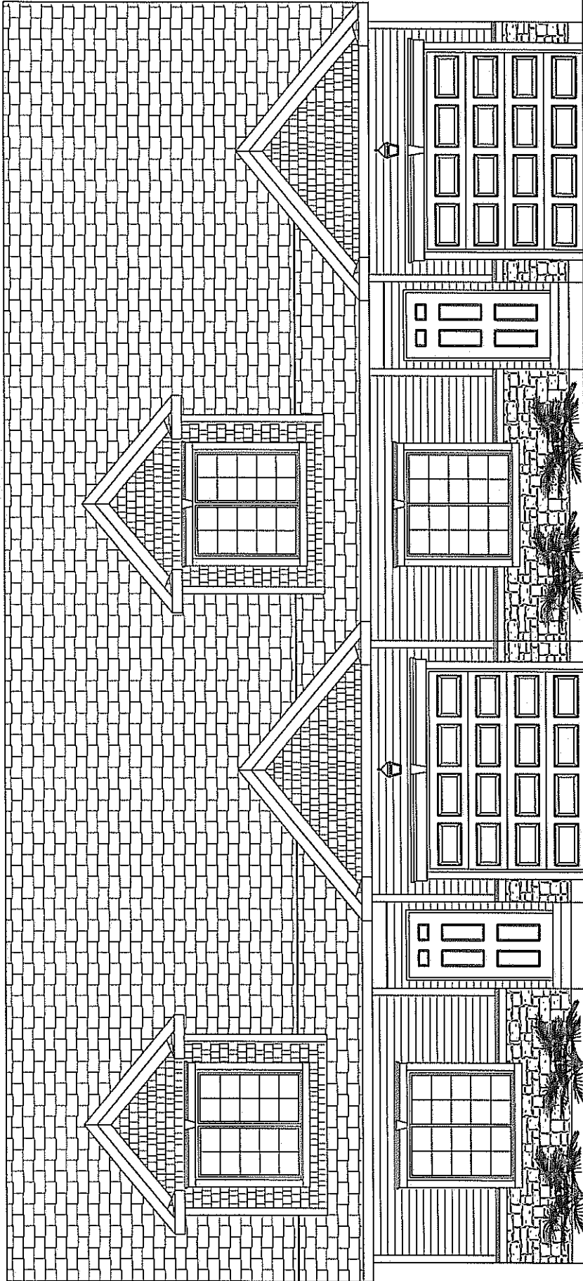
FRONT ELEVATION BURKE DURHAM MODEL
