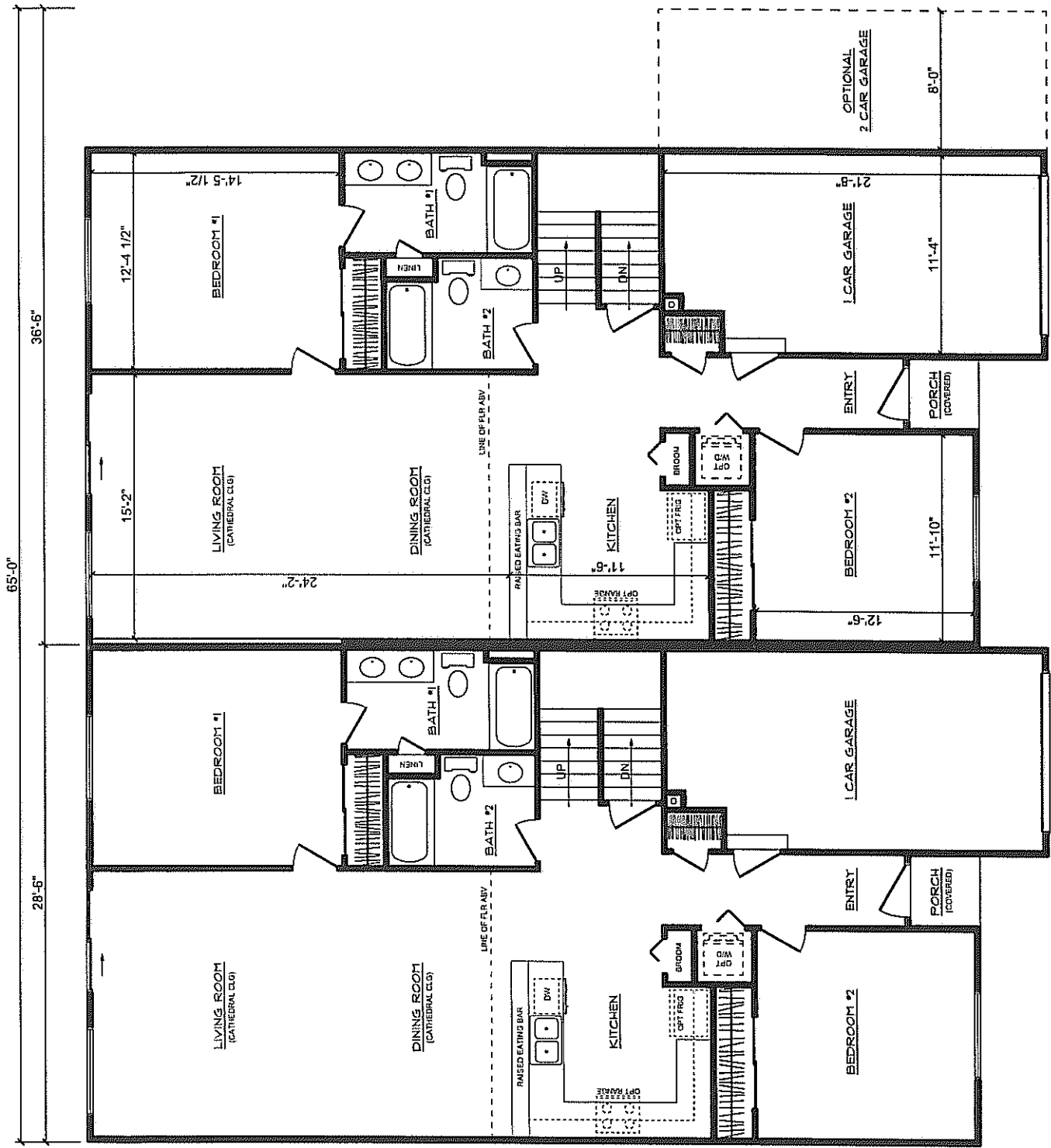
FIRST FLOOR PLAN BURKE DURHAM MODEL BROMPTON TOWNHOMES
