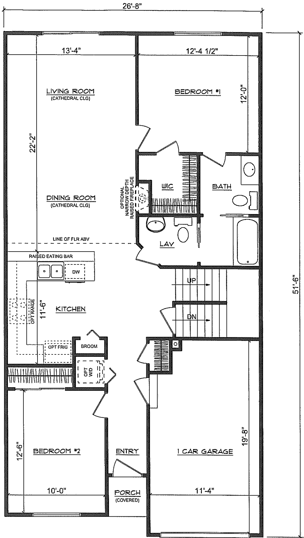
FIRST FLOOR PLAN BURKE COVENTRY MODEL BROMPTON TOWNHOMES
