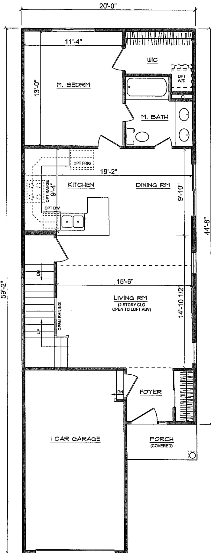
FIRST FLOOR PLAN BURKE AMBERWOOD MODEL BROMPTON TOWNHOMES
