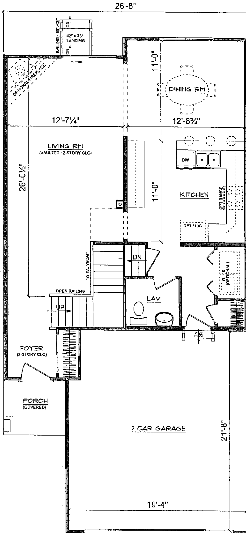
FIRST FLOOR PLAN Burke Bedford I Model
