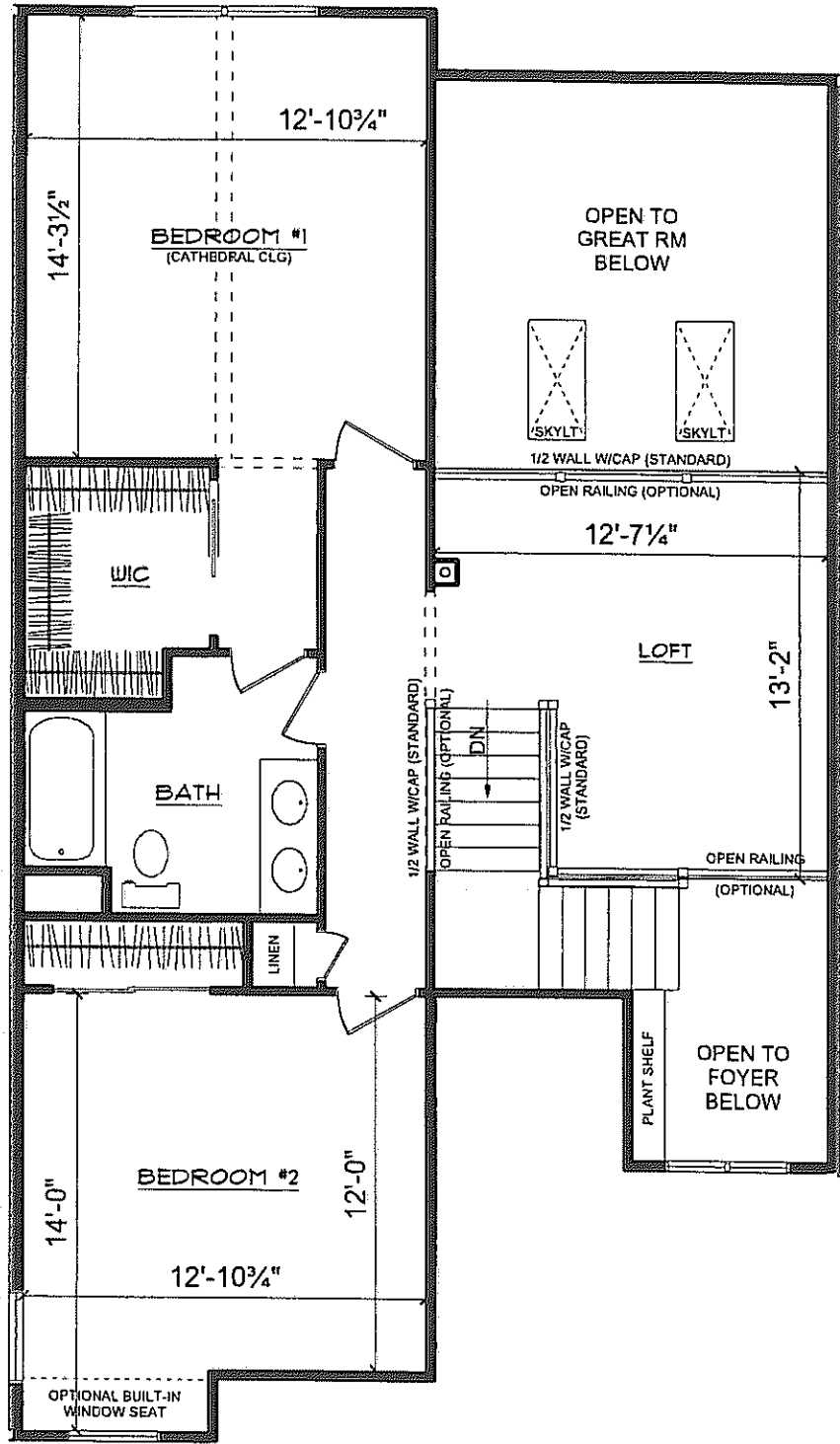
SECOND FLOOR PLAN Burke Bedford 99 Model
