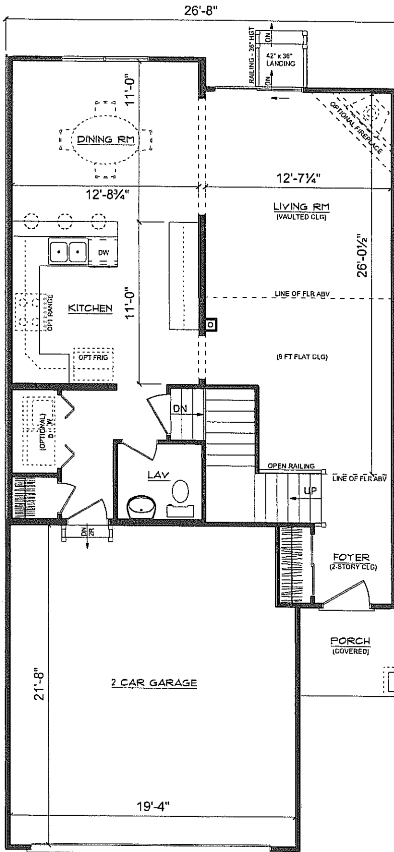
FIRST FLOOR PLAN Burke Bedford II Model
